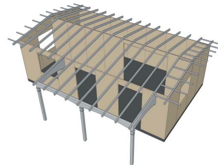
CONSTRUCTION DIAGRAM
