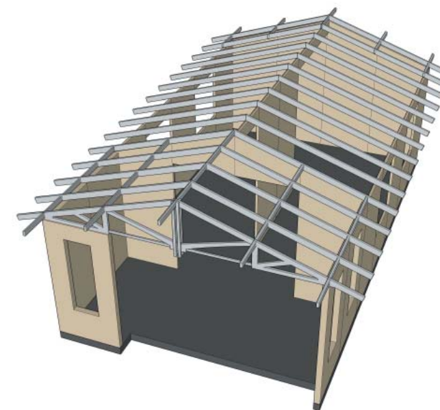
CONSTRUCTION DIAGRAM
