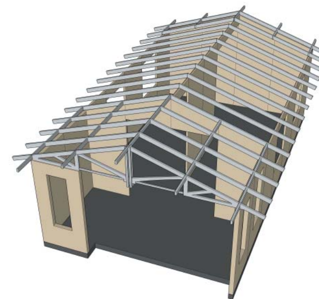
CONSTRUCTION DIAGRAM
